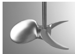
Lightnin A310, A100 and folding Impellers
