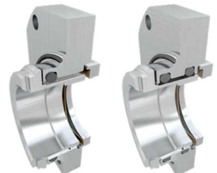
Single and Double O-ring Seal
