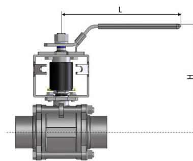
DN65 - DN100; 2,5" - 4"
