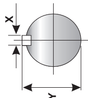
Keyway details Drivfeder detalje
