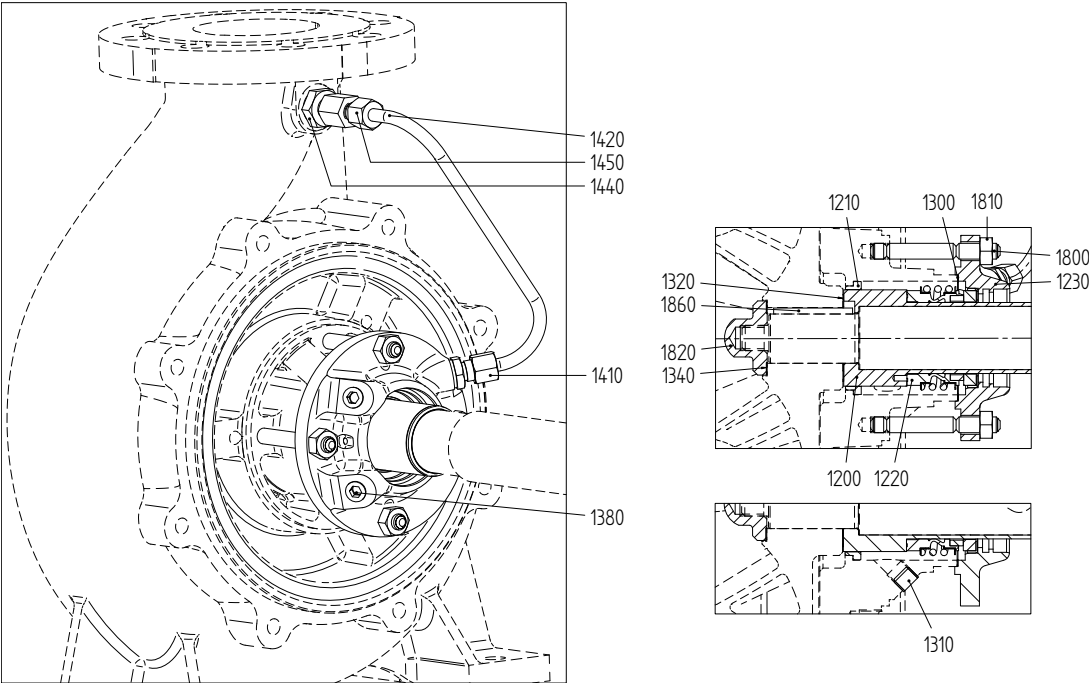
Figure 71: Mechanical seal MG12-G60.
