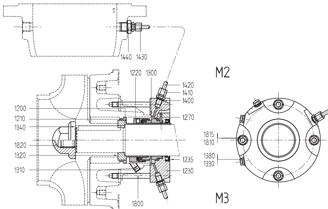
Figure 79: Mechanical seal M2-M3 - bearing group 4.
