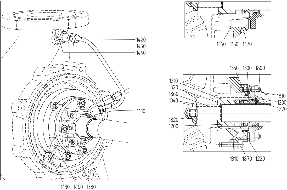
Figure 89: Mechanical seal MW2 - M7N.
