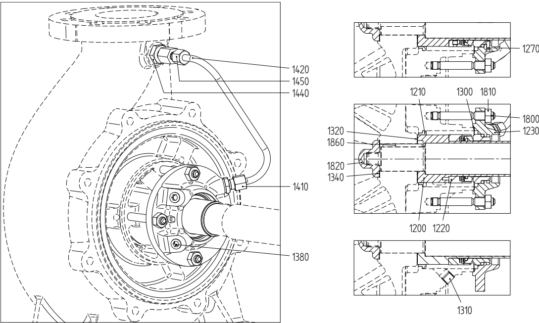
Figure 70: Mechanical seal M7N.
