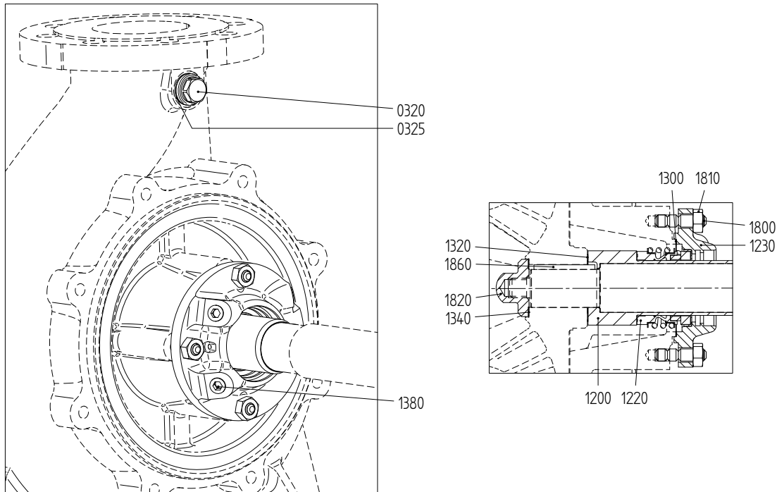
Figure 73: Mechanical seal MG12-G60.
