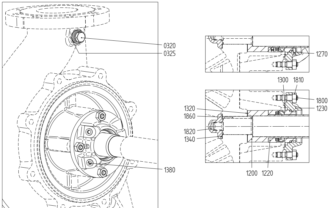
Figure 72: Mechanical seal M7N.
