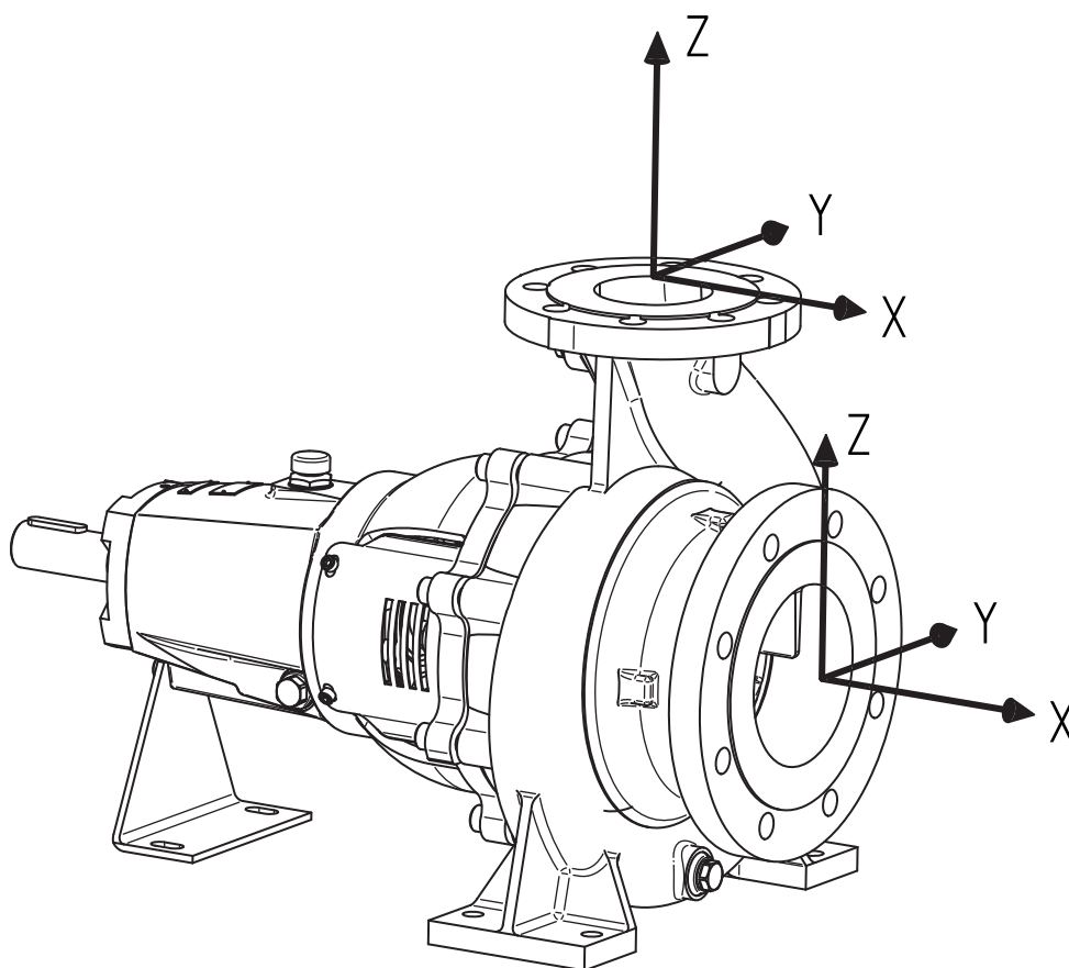
Figure 103: Coordinate system.
