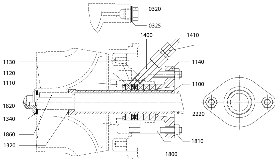
Figure 61: Stuffing box packing S3 for 200-160 / 300-200.
