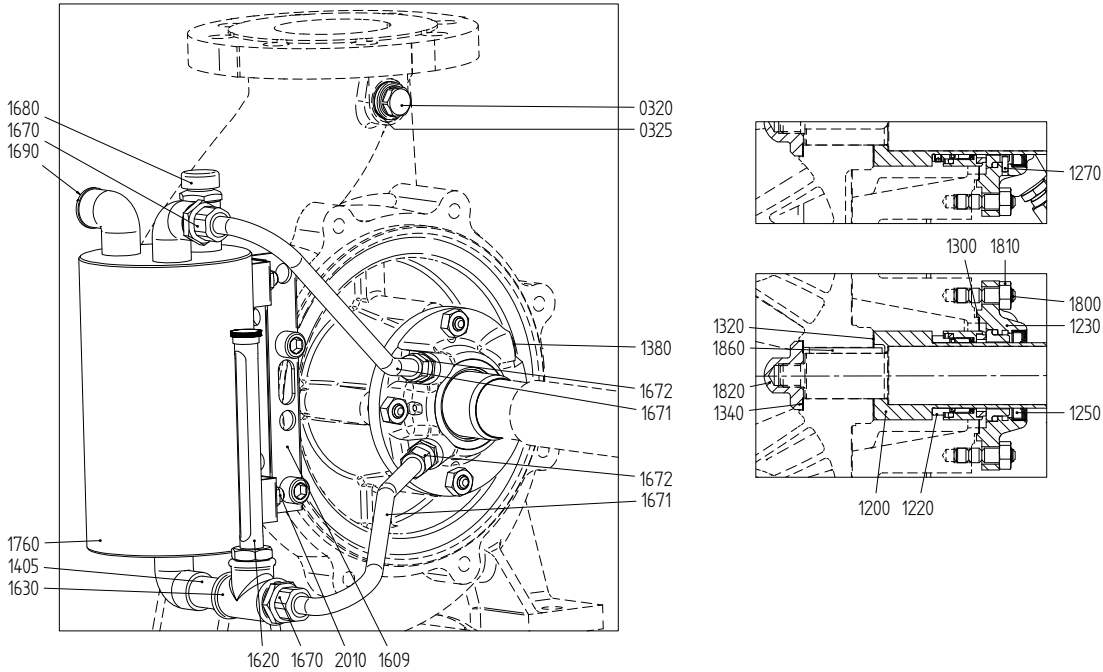
Figure 87: Mechanical seal MQ3 - HJ92N.
