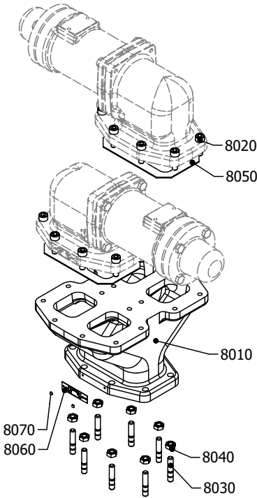
Double safety relief valve – horizontal
