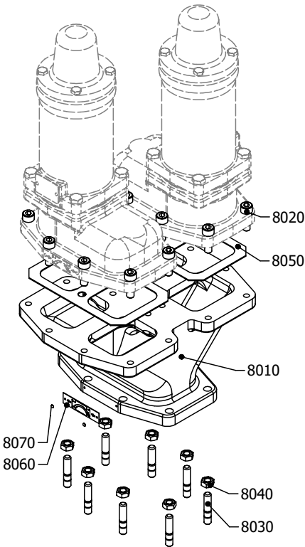
Double safety relief valve – vertical
