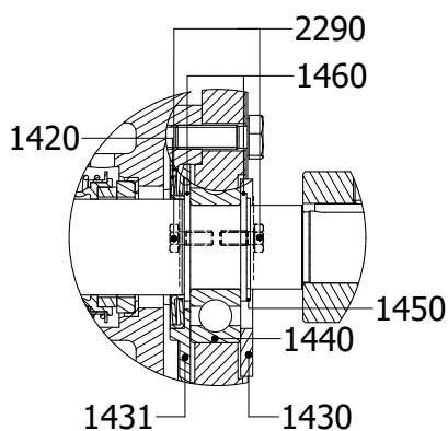
DETAIL B: 15-50 / 23-65
