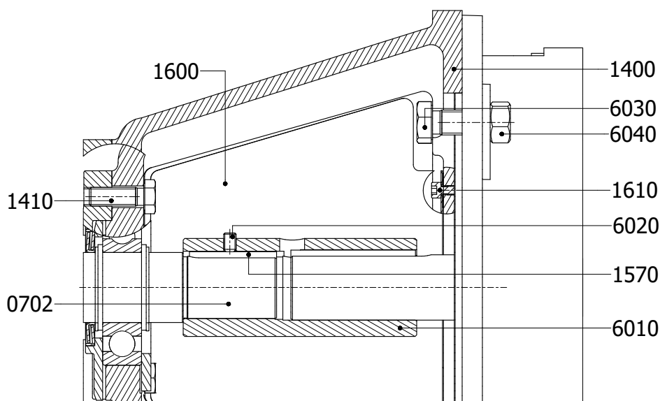
DETAIL B: 15-50 / 23-65
