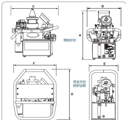
PA60APF5FP (带压力表)
